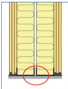
Figure 5.14. Insufficiently separated wall frames (insufficient distance between linings or rigid connection through e.g. thin slabs) as an example of a typical design error.
