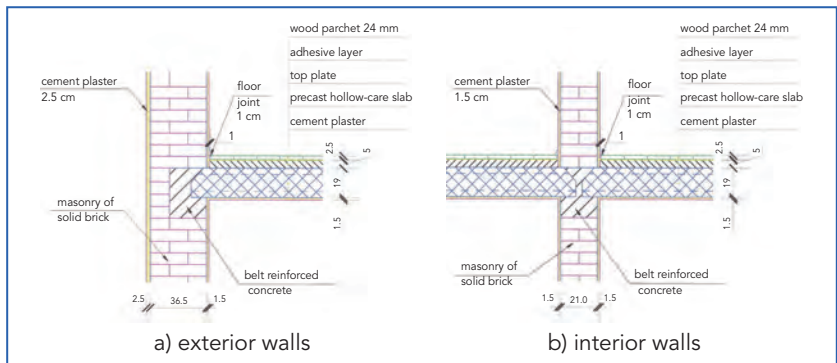
Figure 21.22. Typical details for a floor made of precast reinforced hollow concrete-core slabs and structural walls.
