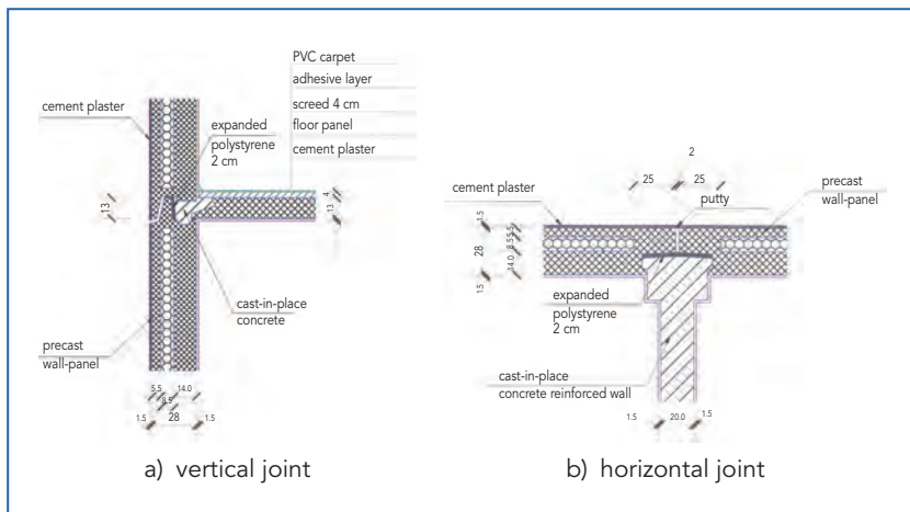
Figure 21.18. Typical details for joints between precast exterior wall panels and slabs.
