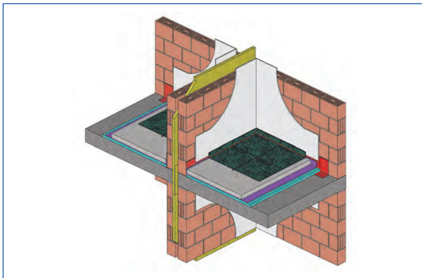
Figure 2.5. Building concept 2 uses semi-heavy walls (> 125 kg/m 2 ) and needs very heavy concrete slabs (> 550 kg/m 2 ) if used for apartment constructions.
