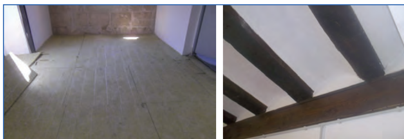
Figure 25.26. Left. Image of the construction of the floating floor. Note that the flanking strips are missing in this image. Right, view of the bottom face of the floor after the retrofitting.
