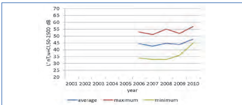
Figure 1.22. L'_{nT,w} + C_{i,50-2500} between flats one above each other.
