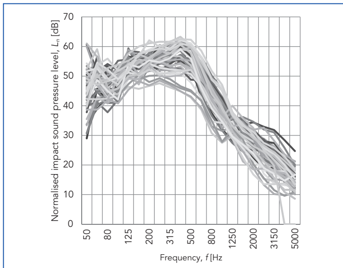
Figure 7.5. Typical impact sound insulation in apartments. Measured in vertical direction. Floor: parquet, Tuplex, hollow-core slab + smoothing compound. L_{n,w} = 40 \dots 55 \text{ dB} [4].
