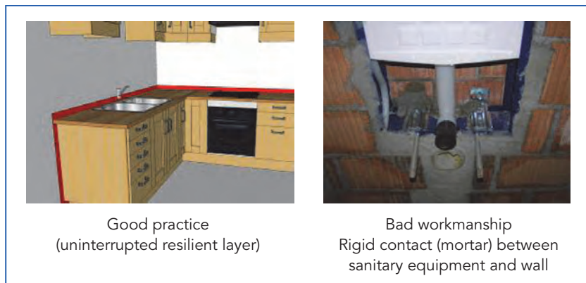
Figure 27.27. Good practice and bad workmanship for service equipment fixation.
