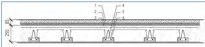
Figure 23.30. Cross-section of ceiling from reinforced concrete with floating floor on the top of it [10].
