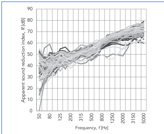
Figure 7.9. Typical airborne sound insulation in apartments. Measured in horizontal direction. Wall: concrete 200 mm. R_w^* = 49 \dots 63 dB [4].
