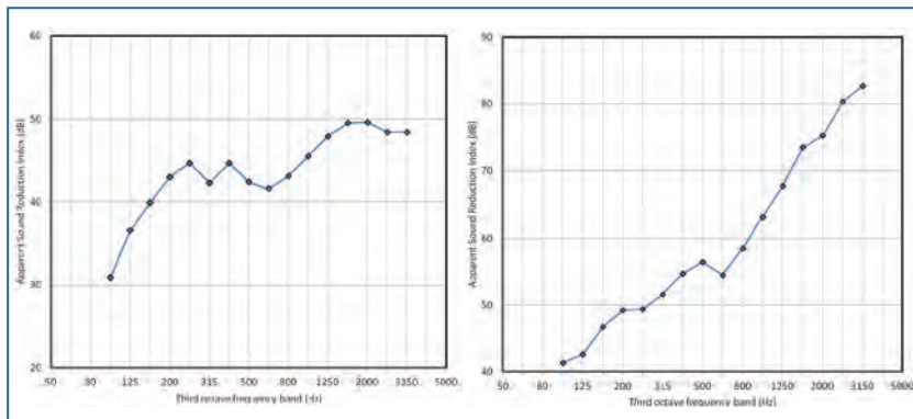
Figure 4.9. Apparent Sound Reduction Index measured in residential building from 1873, 150 mm solid bricks wall with R'_w = 46 dB (left), traditional wooden beam floor with R'_w = 60 dB (right)
