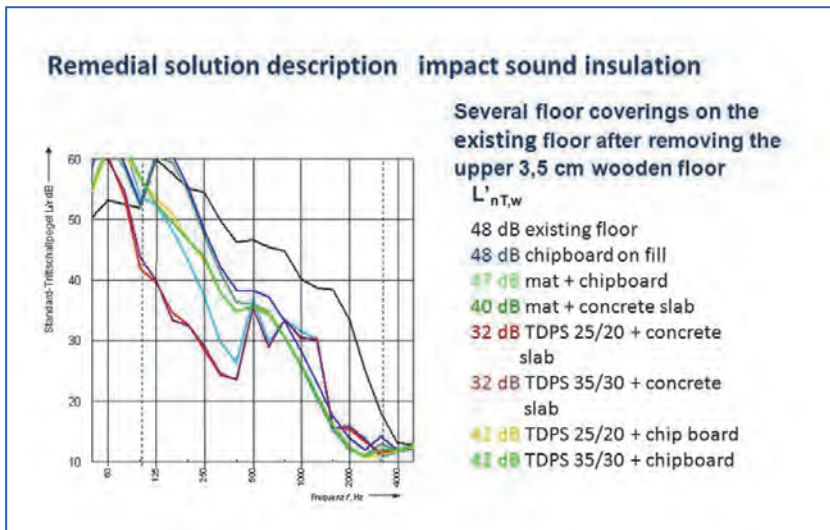
Figure 1.31. Impact sound insulation properties of a timber joist floor with different kind of floor coverings, existing upper floor covering was removed.
