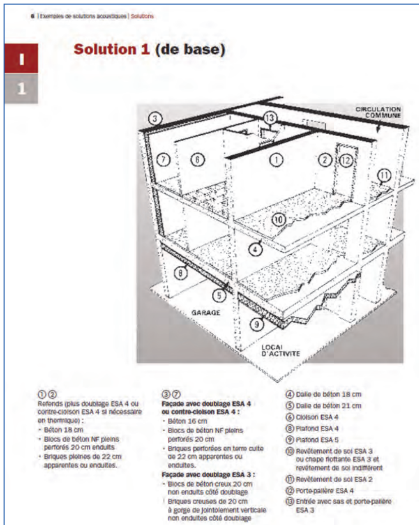
Figure 8.7. Example of building solution from 2002 ESA guide.
