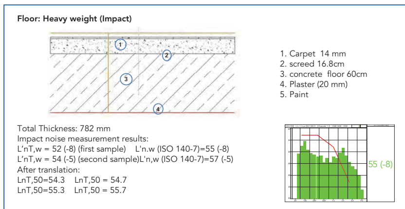
Figure 28.17. Heavy-weight floor. Construction details and impact sound insulation data.
