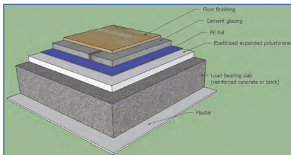
Figure 3.9. Typical cross-section of a modern floor construction.
