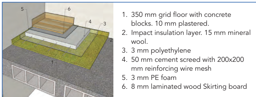
Figure 25.16. Example of a typical Spanish floor.
