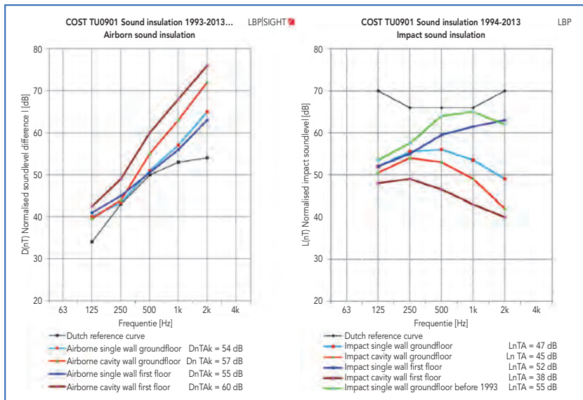
Figure 17.5. Average sound insulation in horizontal direction of newly built terraced houses with solid and cavity walls: airborne (left) and impact (right) for the ground floor and the first floor. (Green line: ground floor with old detail (<1994).
