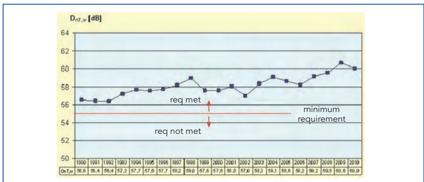
Figure 1.25. Average weighted standardized sound level difference D_{nT,w} between flats one above the other per year.
