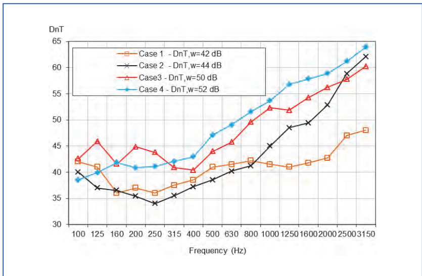
Figure 20.10. Case study: airborne sound insulation of partition walls. Case 1- sprayed plaster, empty cavity; Case 2 – sprayed plaster, insulated cavity; Case 3 – traditional plaster, insulated cavity; Case 4- traditional plaster on both sides and on one cavity face, plus insulated cavity.
