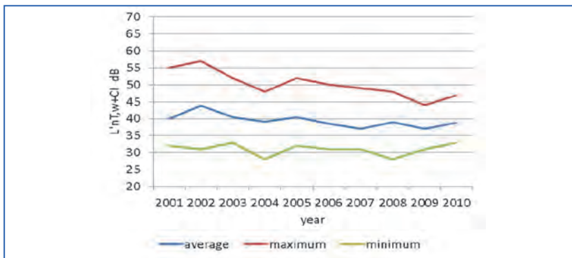
Figure 1.21. L'_{nT,w} + C_i between flats one above the other.
