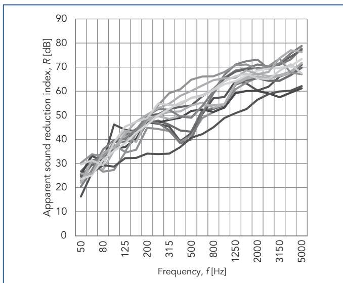
Figure 7.10. Typical airborne sound insulation in apartments. Measured in horizontal direction. Wall: lightweight structure. R_w^* = 45 \dots 62 dB [4].
