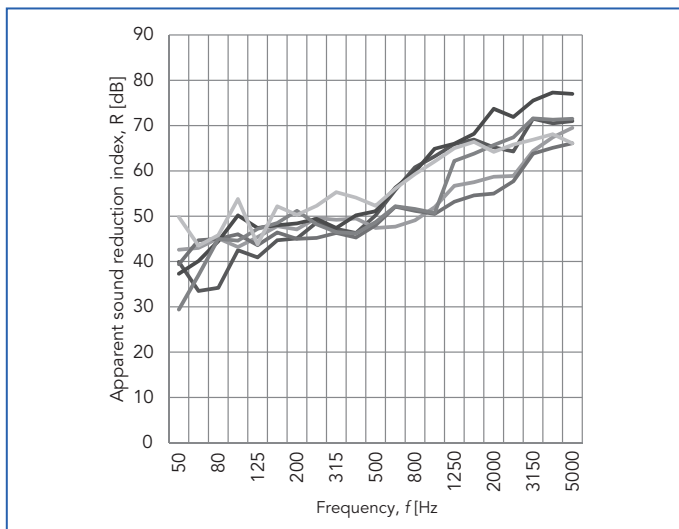
Figure 7.8. Typical airborne sound insulation in apartments. Measured in vertical direction. Floor: parquet, Tuplex, massive concrete slab + smoothing compound. R_w = 52 \dots 60 dB [4].
