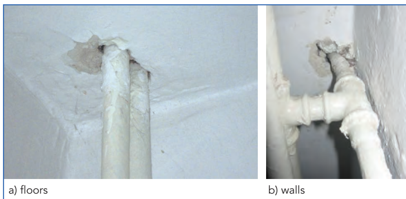
Figure 21.21. Typical errors for cross pipes.
