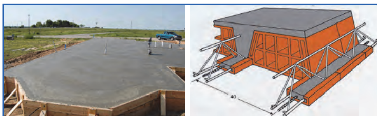
Figure 15.6. Floor structures: a) solid reinforced concrete slab; b) beam and block floor (semi-prefabricated floor), type “Monta”.
