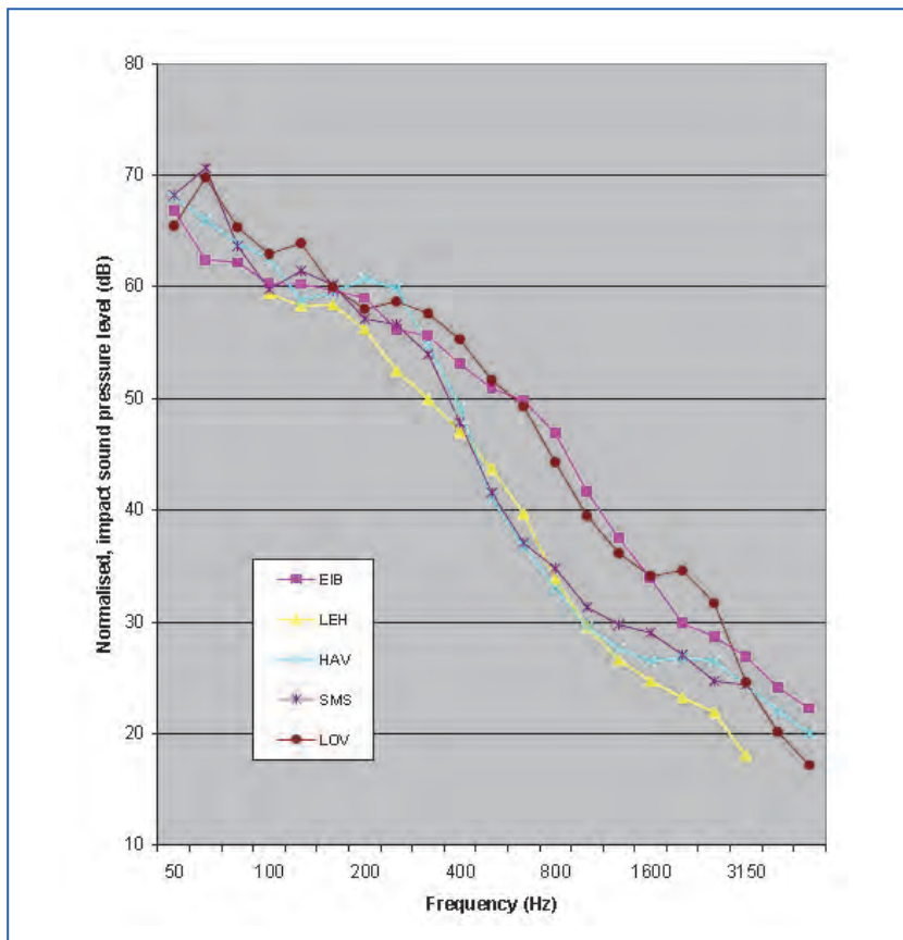
Figure 18.4. Typical impact sound pressure levels on various lightweight wooden floors [7], as described in the text above.
