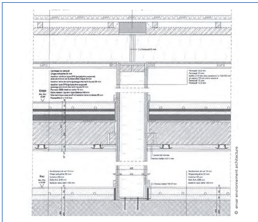
Figure 27.13. Quality lightweight construction designed to fulfill Swiss increased requirements.
