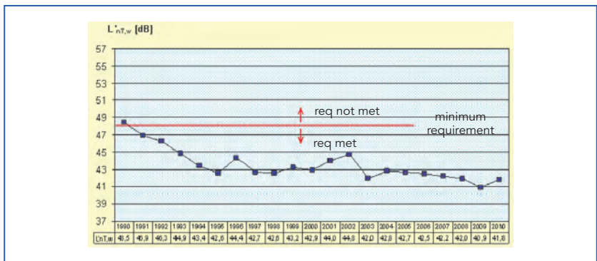
Figure 1.27. Average weighted standardized impact sound pressure level L'_{nT,w} of floors between flats per year.
