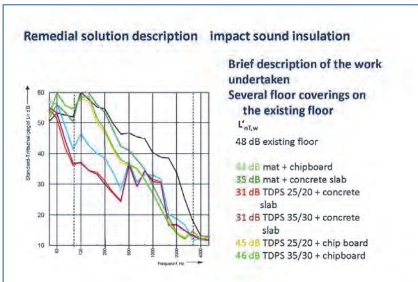
Figure 1.32. Impact sound insulation properties of a timber joist floor with different kind of floor coverings, added to the existing floor covering.
