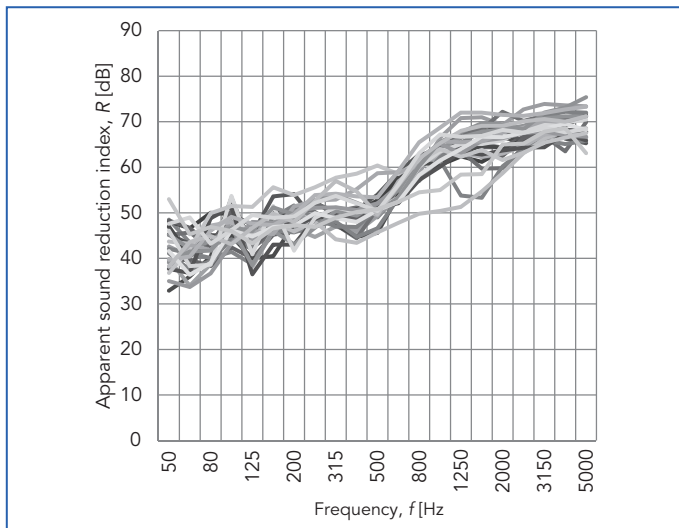
Figure 7.7. Typical airborne sound insulation in apartments. Measured in vertical direction. Floor: parquet, Tuplex, hollow-core slab + smoothing compound. R_w = 51 \dots 62 dB [4].
