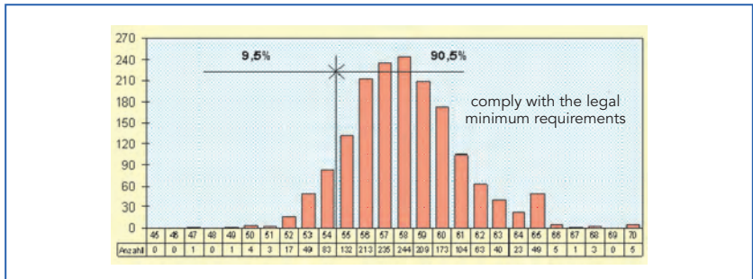
Figure 1.26. Frequency of weighted standardized sound level difference values between flats one above the other (measured during the period from 1990 – 2010).
