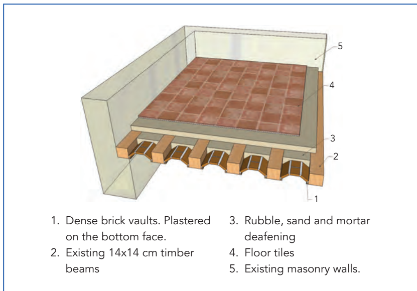
Figure 25.21. Typical floor dating 1900's. It is composed of a series of wooden beams, 14x14 cm in average. Bricks were laid between the wooden beams forming a vault and a rubble infilling was placed on top. The floor was tiled or wooden.
