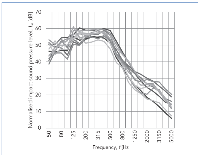
Figure 7.6. Typical impact sound insulation in apartments. Measured in vertical direction. Floor: parquet, Tuplex, massive concrete slab + smoothing compound. L_{n,w} = 47 \dots 53 \text{ dB} [4].
