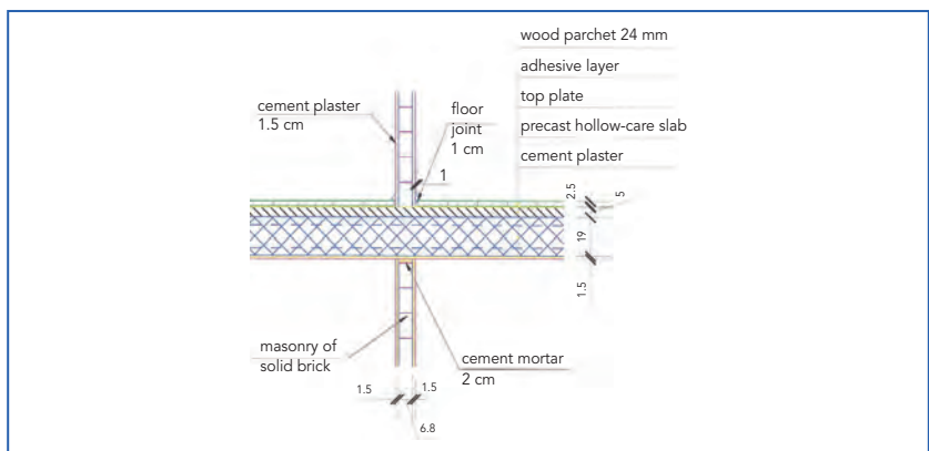
Figure 21.23. Typical details for a floor made of precast hollow reinforced concrete-core slabs and inner walls.
