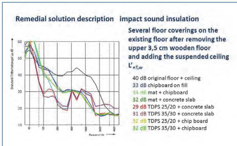
Figure 1.33. Impact sound insulation properties of a timber joist floor with different kind of floor coverings, added to the existing floor covering and suspended ceiling.
