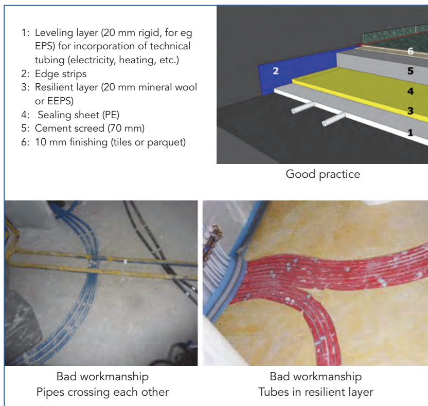
Figure 27.21. Good practice and bad workmanship for heavy floating floors (screed).
