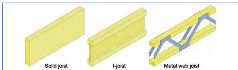
Figure 29.9. Examples of separating floor joists used in the UK.
