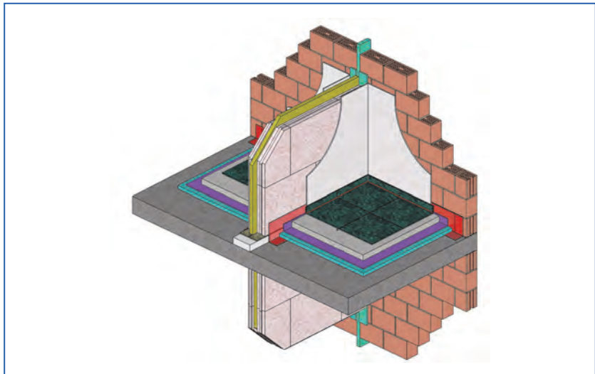
Figure 2.20. Sketchup drawing of building concept 8.
