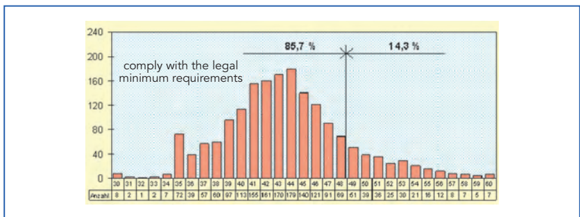
Figure 1.28. Frequency of weighted standardized impact sound pressure level values between flats one above the other (measured during the period from 1990 – 2010).
