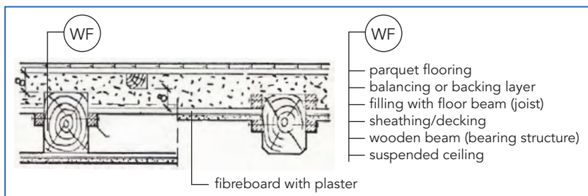
Figure 23.5. Composition of original wood flooring (WF) [7].
