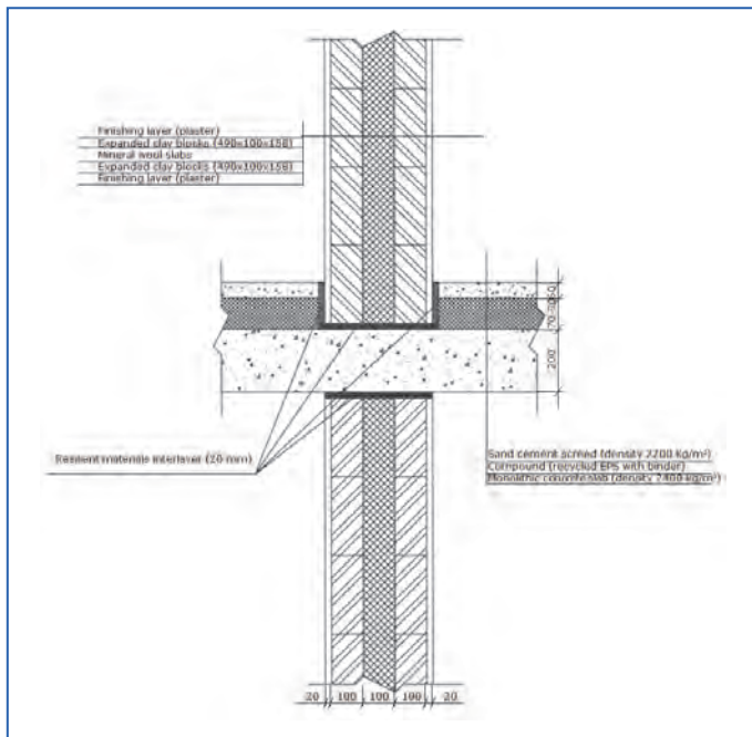
Figure 14.2. Separating wall connection with separating floor.
