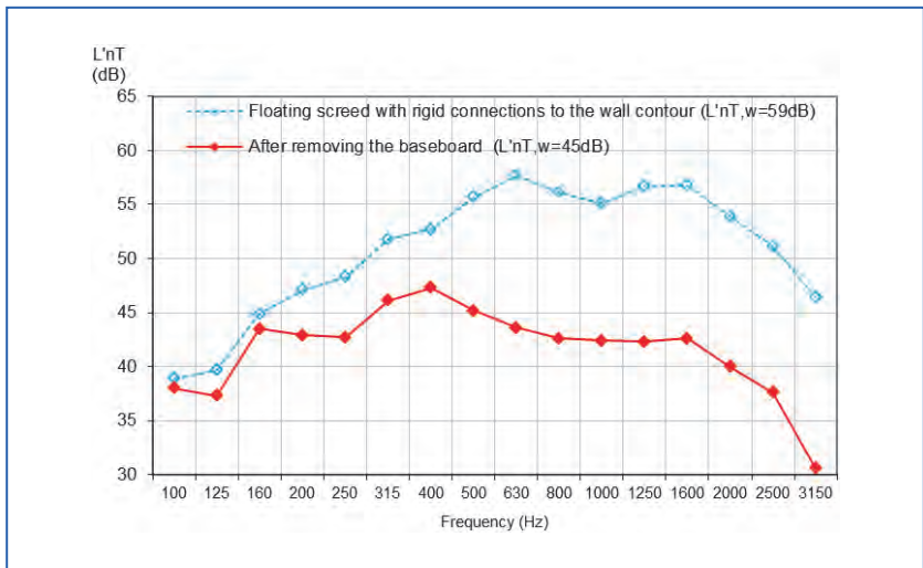
Figure 20.11. Case study: Vertical measurements of impact sound transmission (upward), before and after removing the baseboard.
