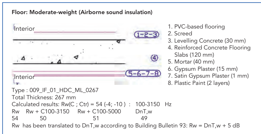
Figure 28.16. Moderate-weight floor. Construction details and airborne sound insulation data.
