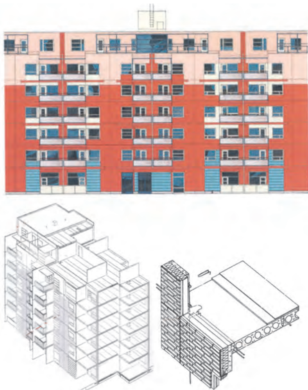
Figure 7.17. Example of a dwelling constructed in 1986. Top: façade 1:250, bottom left: cross section, bottom right: junction between exterior wall (concrete sandwich element) and floor (hollow-core slab 265 mm). Typical structures: floor: hollow-core slab 265 mm, walls between dwellings: concrete 180 mm [5].
