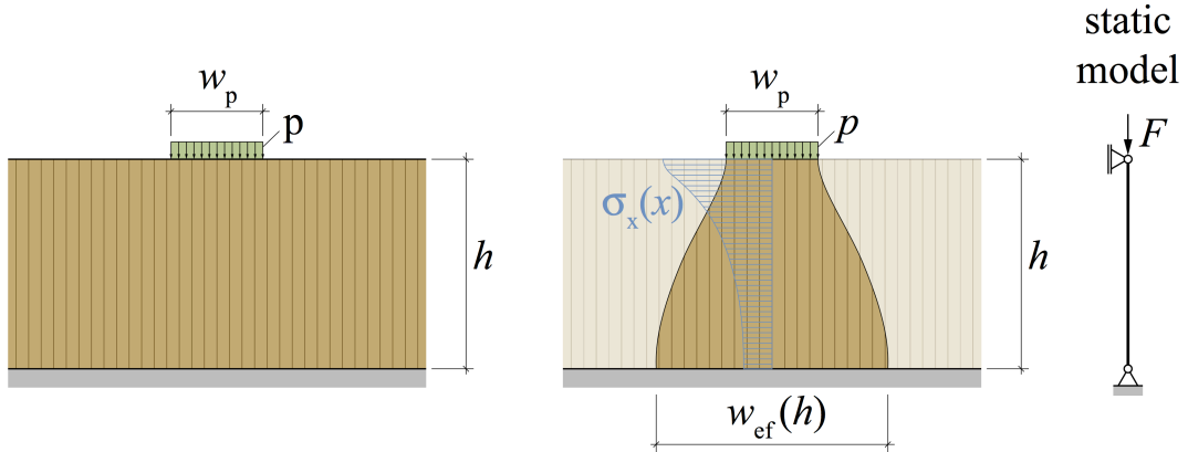
Fig. 11 CLT wall with local load p uniformly distributed over the length w_p , the effective load distribution width w_{\text{ef}}(x) , the stress distribution \sigma_x(x) along the axis of symmetry and over the diaphragm's height h as well as the static model.
