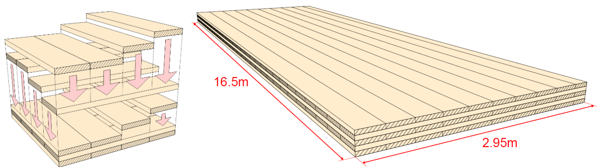
Fig. 1 Cross-Laminated Timber.
