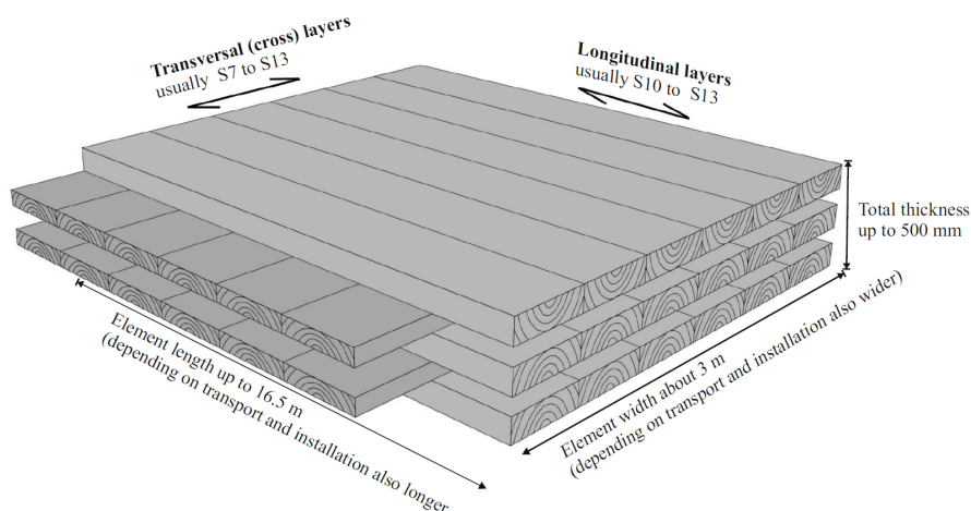
Fig. 1 Sketch of a cross-laminated timber panel. In this paper, longitudinal layers and load-bearing layers are used interchangeable.
