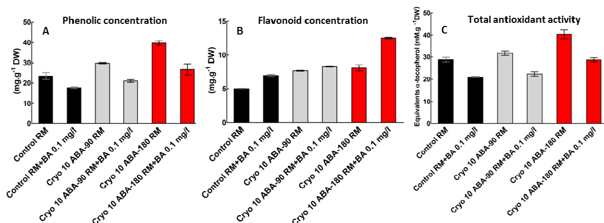
Fig.2. Influence of cryopreservation on the secondary metabolites accumulation in regenerated Hypericum rumeliacum plants. Error bars indicate \pm SEM (n-1)
